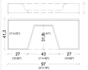
TOP VIEW DRAWER
