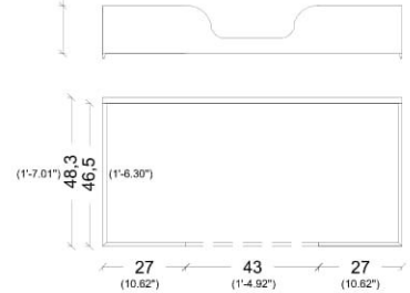
TOP VIEW DRAWER
