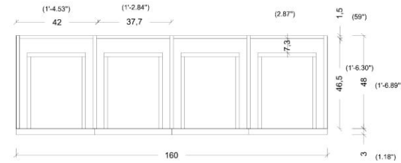
BACK VIEW DRAWER
