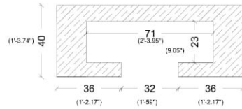
BACK VIEW
